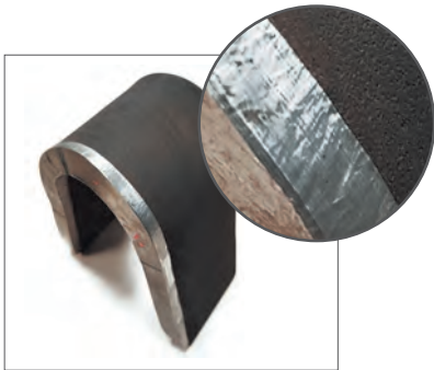
180° side bend sample for Ni-625 cladding with Hybrid Technique
